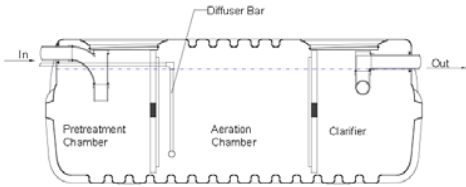
The CajunAire Advanced Flow Diagram (Poly)
