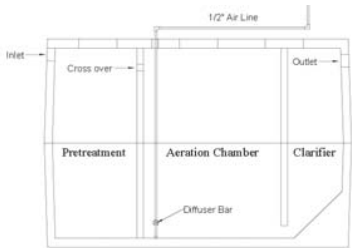
The CajunAire Advanced Flow Diagram
